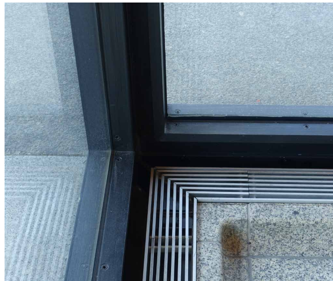
FIG. 5.40 New National Gallery, Berlin: New facade with a single glazing in a thermally non-separated construction / Photo: F. May
