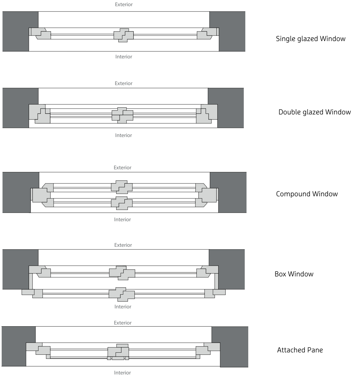
FIG. 5.20 Basic single and double glazed wood window constructions
