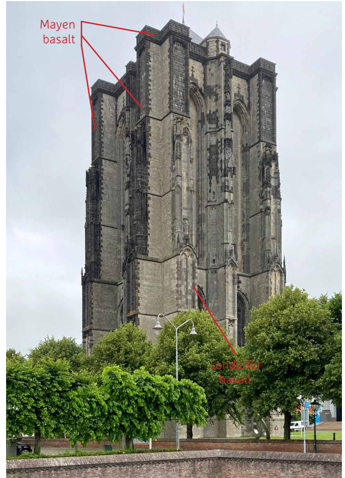
FIG. 2.5 Londorfer basalt was used as a replacement stone in the lower section of the south side of the Lievensmonster Tower in Zierikzee. At the top and on the west side, mainly Mayen basalt can be seen / Photo: W.J. Quist
