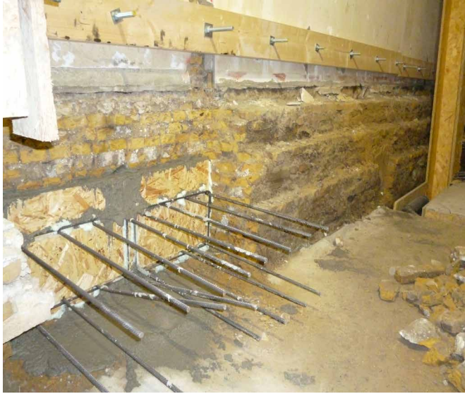
FIG. 3.10 Huis Nolet, basement: reinforcement for insertion of concrete floor (December 2016) / Photo: B. L.ubelli
