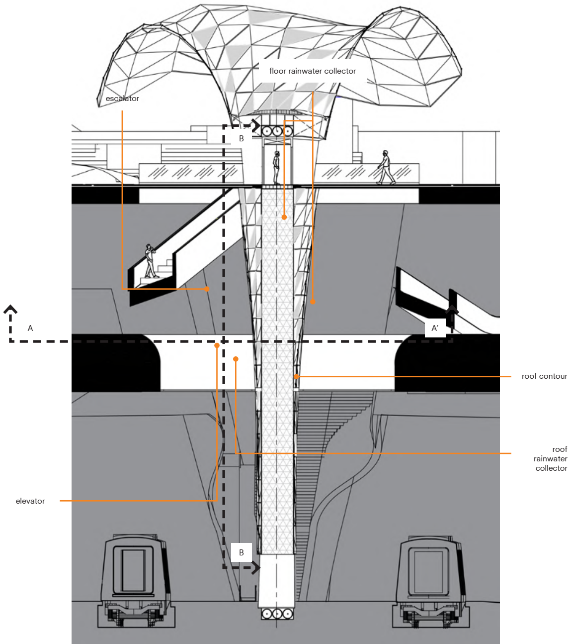
The "Mushroom" Section A-A'
