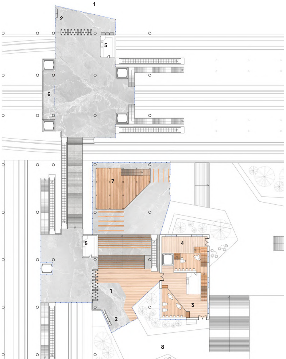
1. Station gates; 2. Ticket point; 3. Cafeteria; 4. Library; 5. Kiosk; 6.Store; 7.Flexible public space; 8. Public square
