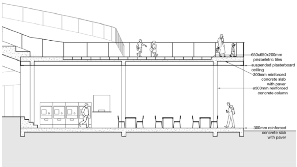
Detailed Section
