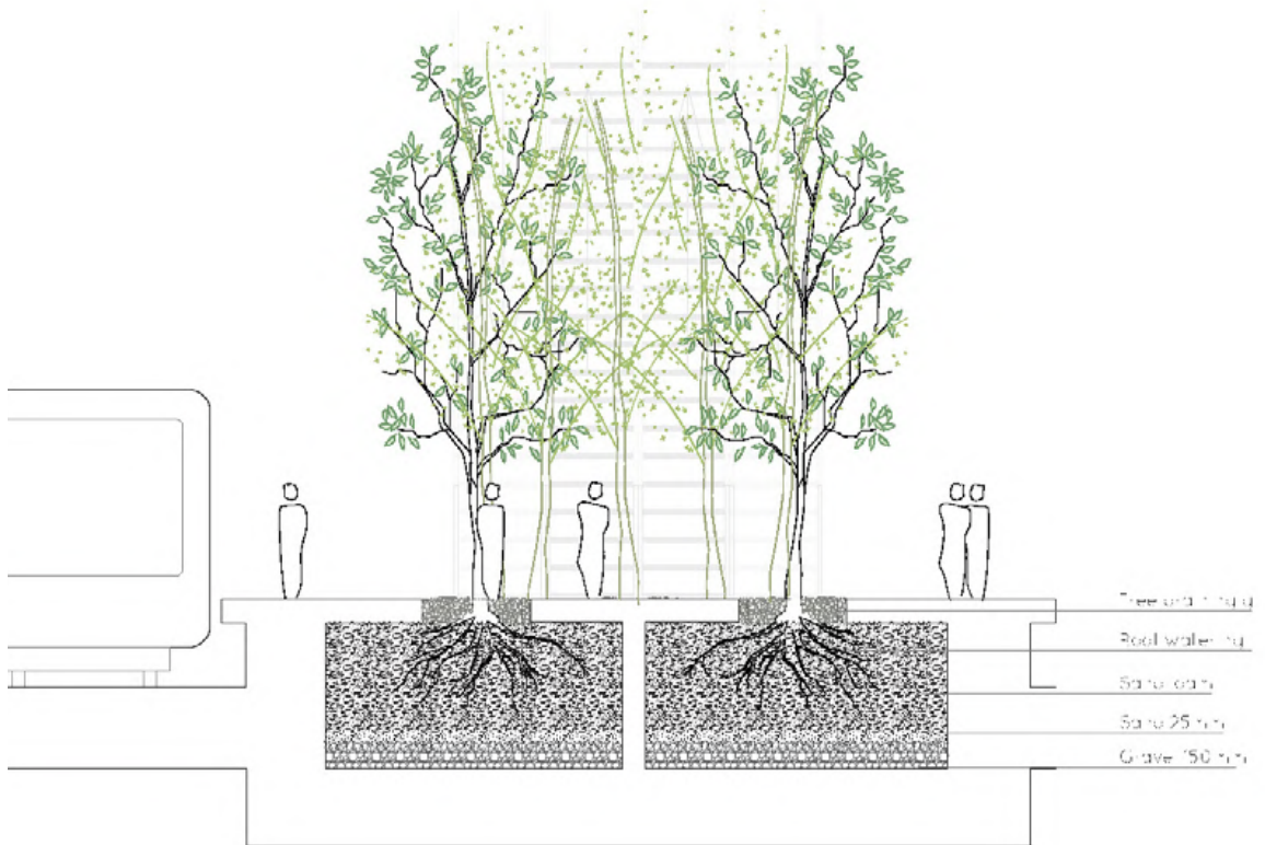
Section of plant beds in the metro platform
