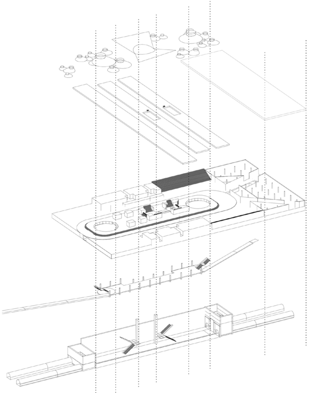
Station and Urban Plaza Exploded Axonometric
