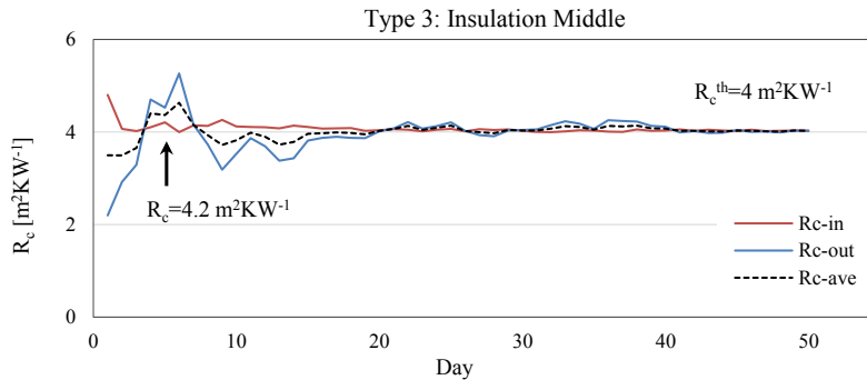
FIG. 2.6 Fig 2.6- R_c -values obtained from the type-3 wall: two homogeneous brick layers connected via insulation in the middle. The effect of the insulation is divided and thus, the side with more stable temperature converges earlier.
