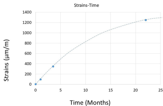
FIGURE 5.30 Strain measurement results of unloaded bridge (only self-weight) of five measurements in time.
