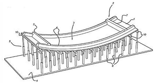
FIGURE 4.6 A flexible mould system for cambered decks with variable width and length.
