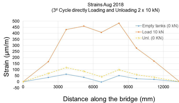
FIGURE 5.27 Third Load Cycle; Results of strains in tension sensors along the bridge (Line 2), Loading and unloading directly to 2x 10,0 kN. The dotted line shows the remaining strains.
