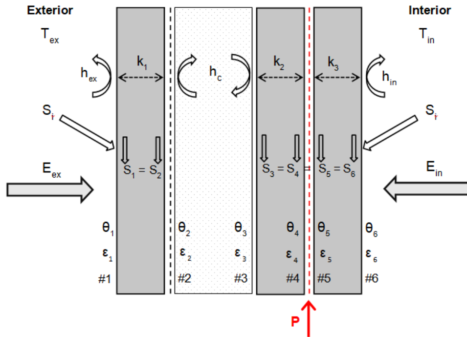
Figure 1 - Radiant glass configuration and variables used in the thermal balance model.
