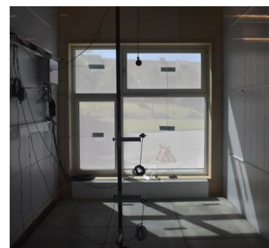
► Fig. 3: View of the inside of one of the twin test cells.
