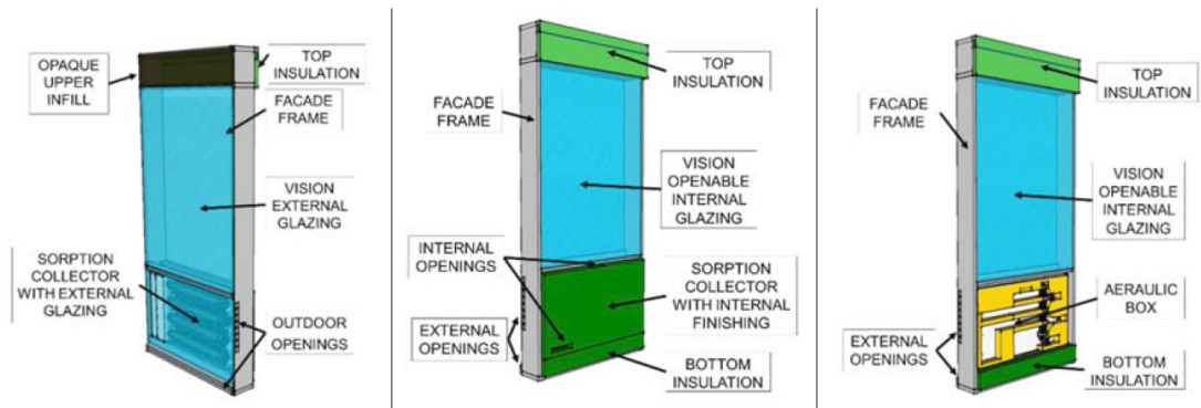
Figure 2 - 3D rendering of the whole assembly of the façade with the sorption collector integrated in the spandrel
