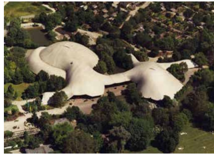
FIGURE 4.18 Figure 4.18: Roof for Multihalle in Mannheim, Germany, 1975 [105].
