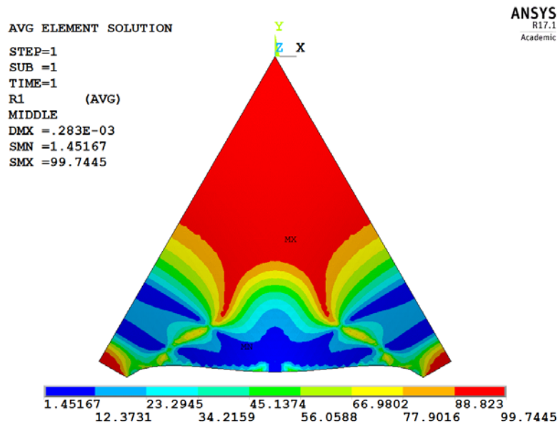
FIGURE 8.30 R_1 of Model A_s (shell with simply supported straight supports) when the shell fails (%).
