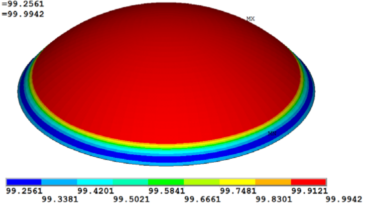
FIGURE 4.16 Strain-energy ratio \alpha of the dome (%).
