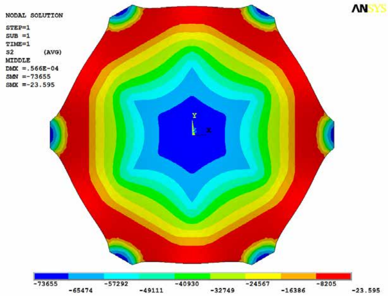
FIGURE 5.21 Principal stress S_2 at the middle surface of the shell of Example 5.2 (Pa).
