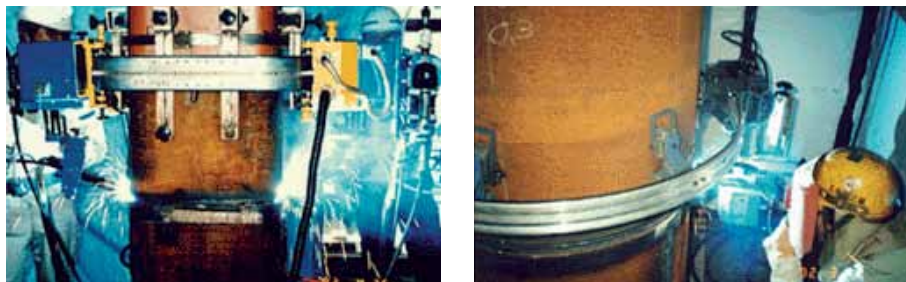
Figure 43 Welding robot, Takenake Corp.
