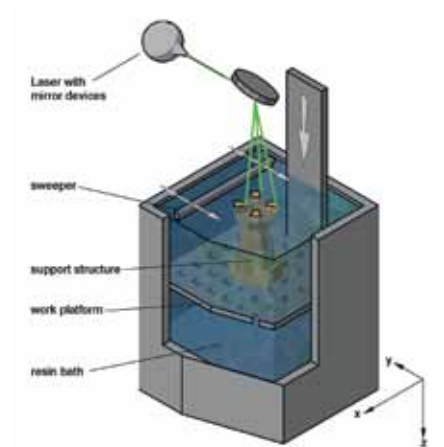
Figure 11 Schematic drawing: SLA method
