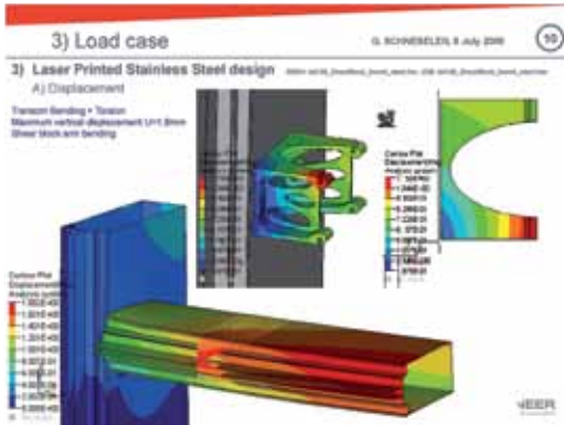
Figure 65 FE-analysis results; conducted by Kawneer-Alcoa during the project.
