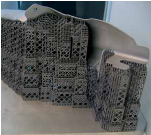
Figure 25 DMLS support structures still attached to the part and substrate plate.
