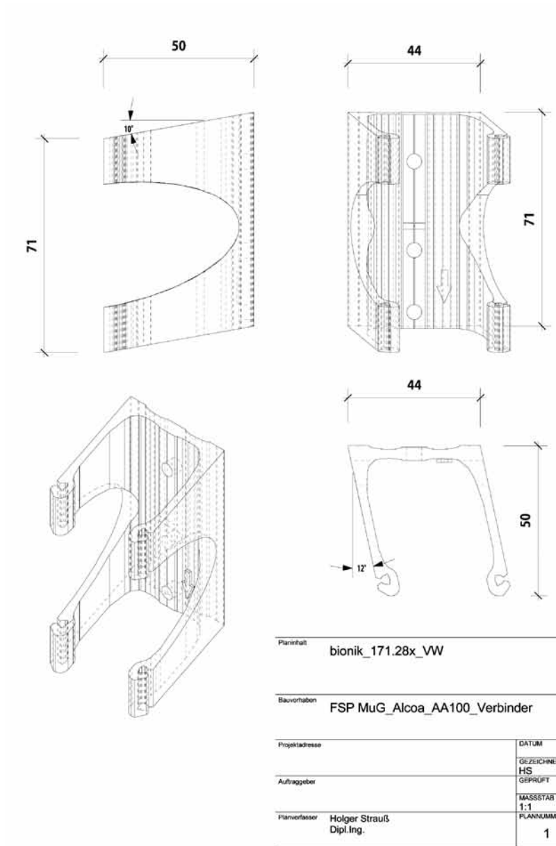
Figure 100 Optimised part as result of the optimisation for AM; in this part material was digitally 'cut off', where it is structurally not needed.
