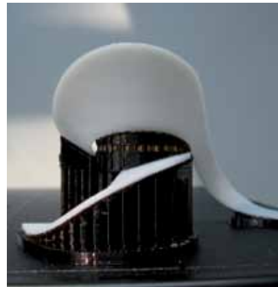
Figure 16 The visible structure of the different layers after completion of the FDM print job. In white: the ABS material; in brown: the soluble support structure
