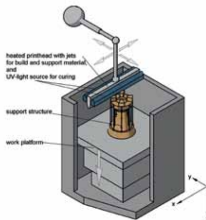
Figure 19 Schematic drawing: PolyJet™ method
