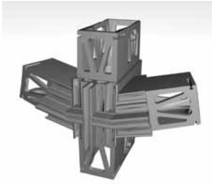
Figure 70 Rendering: NEMATOX II, 3D façade node for Alcoa 'AA-100' façade system.
