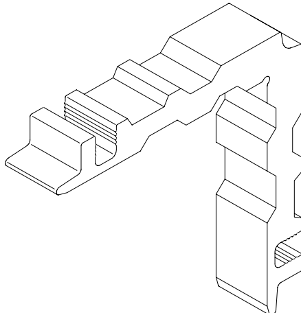
Figure 55 Drawing of standard corner cleat 272.xx from Alcoa e-catalogue.
