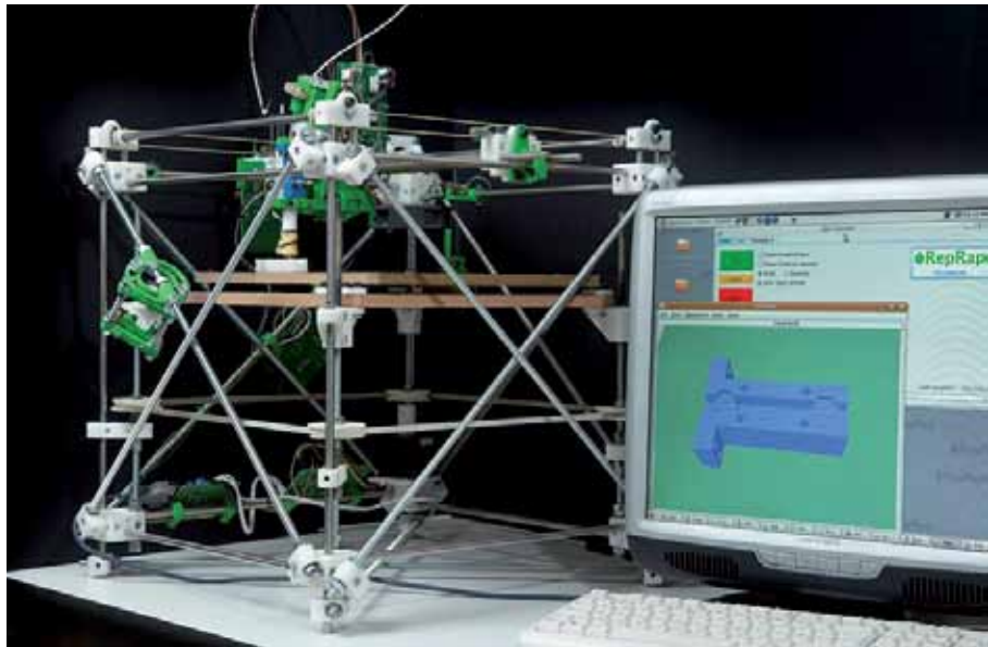
Figure 94 RepRap, Darwin1; Developed at University of Bath, England.
