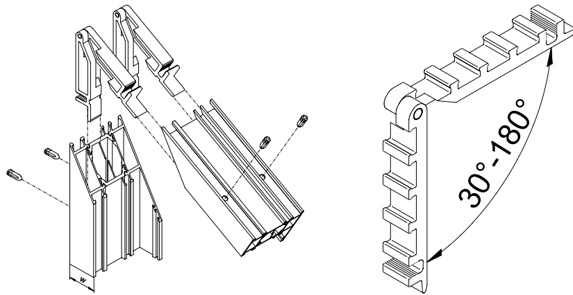
Figure 53 Corner cleats for non-orthogonal window frames; angle manually adjustable; Imagery and illustrations from Kawneer-Alcoa digital catalogue, Issue 10/2010
