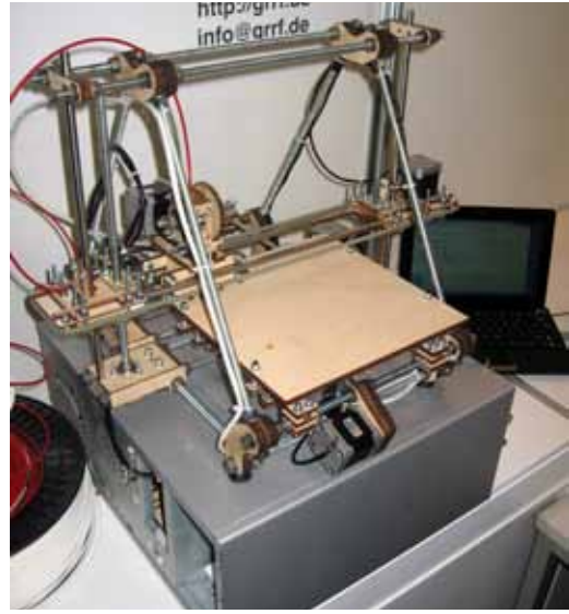
Figure 22 Self-assembled RepRap; FH Darmstadt 2010
