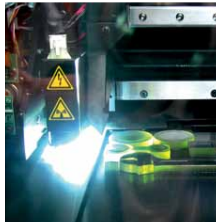
Figure 20 PolyJet process during the UV-light curing of the plastic material on the building platform (below).
