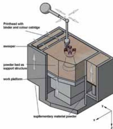
Figure 17 Schematic drawing: 3DP method
