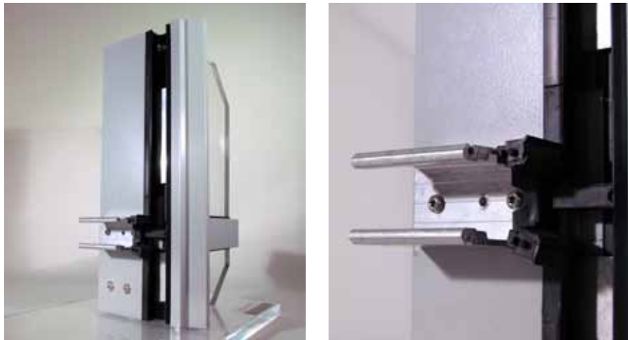
Figure 61 Standard T-connector mounted to AA-100 mock-up.
