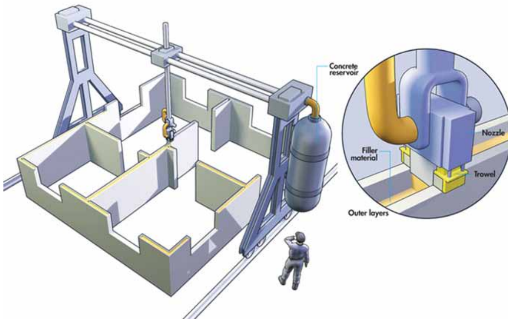
Figure 35 Visualisation of Contour Crafting set-up for the production of housing. Imagery courtesy of B. Khoshnevis.
