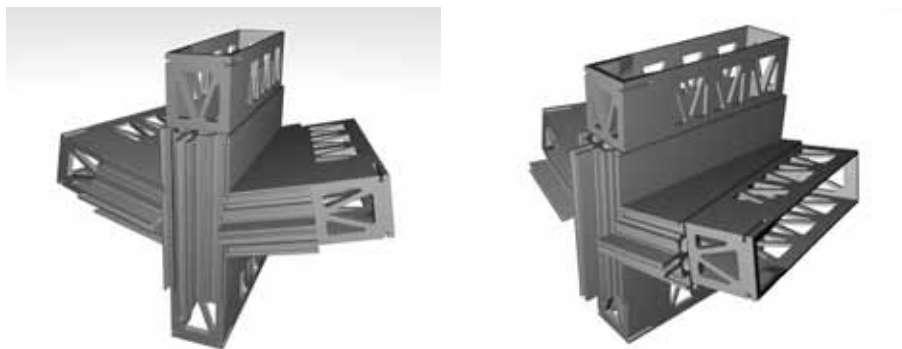
Figure 68 Rendering, NEMATOX I, 3D façade node for Alcoa 'Next' façade system.
