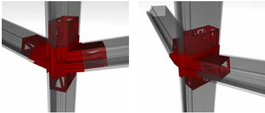
Figure 69 Principle of construction for façade node within a façade system; all angles can be digitally adjusted to the desired geometry and deformation.
