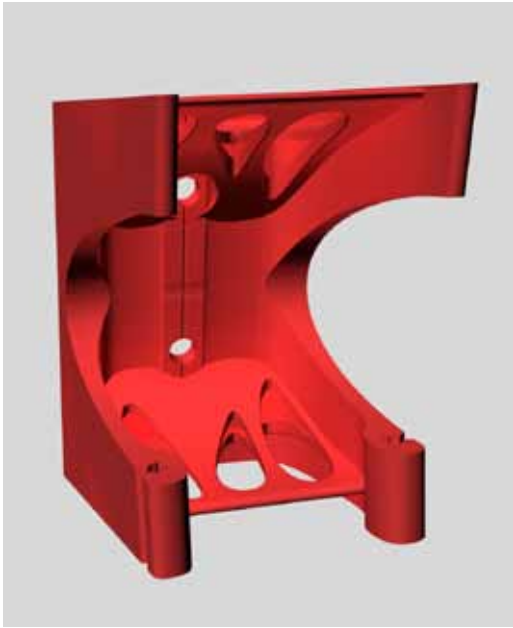
Figure 63 3D connector: rendering (left), printed part in stainless steel (right), realized on a DMLS system by EOS @ FKM Sintertechnik GmbH
