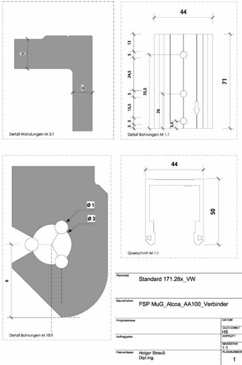
Figure 98 Technical drawing of the standard T-connector for a stick system; details and dimensions for the optimisation process. All screw channels and technical features were re-constructed in the advanced connector.
