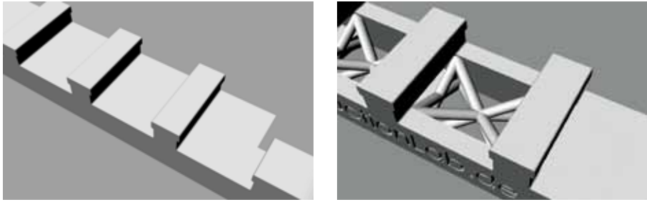
Figure 54 Rendering of 271.xx, detail; left: standard solution digitally drawn from e-catalogue; right: AM optimized solution; digitally reduced material and light weight structures. Digital branding on the side of the part: this could also be used for part identification.
