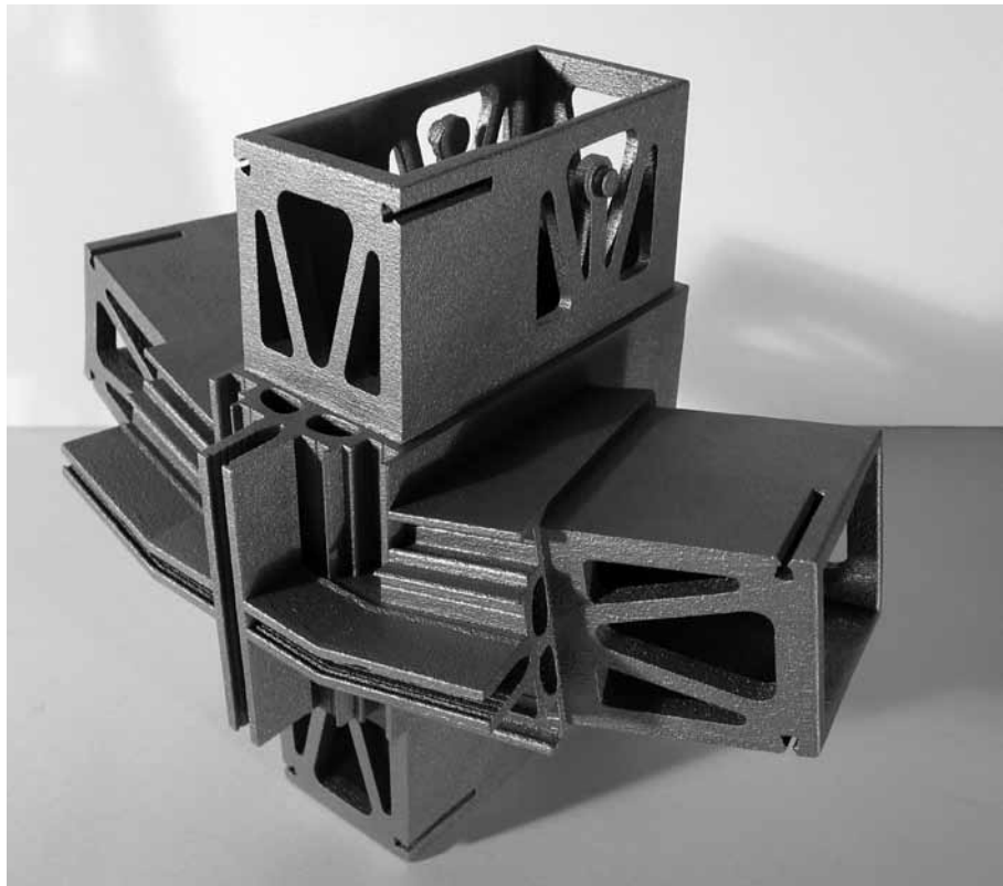
Figure 74 Printed nodal point in aluminium, realized on a ConceptLaser system by EOS @ FKM Sintertechnik GmbH
