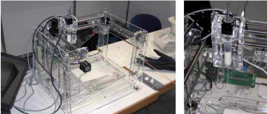
Figure 96 Fab@Home (left); extrusion nozzle (right) with medical syringe as the nozzle device.
