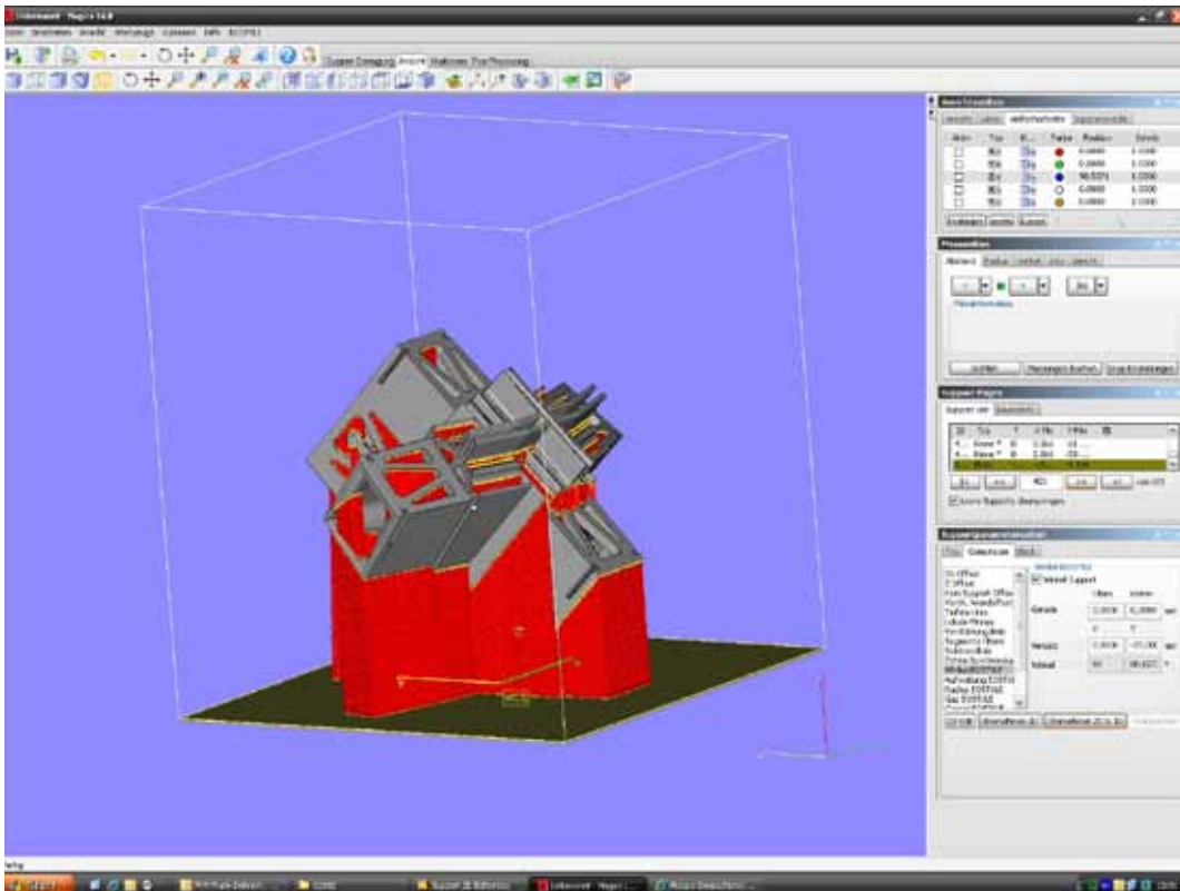
Figure 75 Build job preparation: screenshot of orientation of Nematox II within the DMLS building chamber representation; indicated in red is the needed support structure; @ FKM Sintertechnik GmbH
