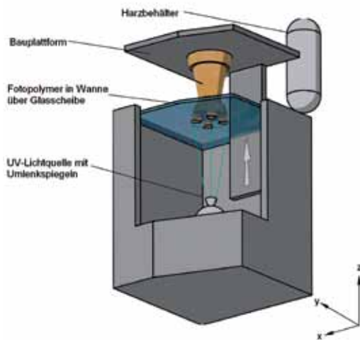
Figure 90 Schematic drawing DLP method
