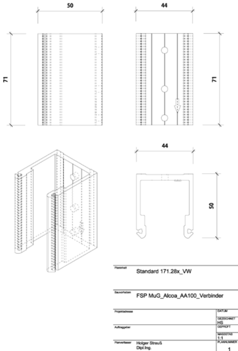
Figure 97 Technical drawing of the standard T-connector for a stick system; used as digital background for optimisation.
