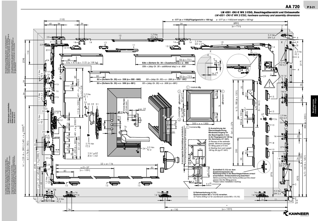
Figure 82 Mounting details for a standard window by Alcoa 'AA-720'. Imagery and illustrations from Kawneer-Alcoa digital catalogue, Issue 10/2010.
