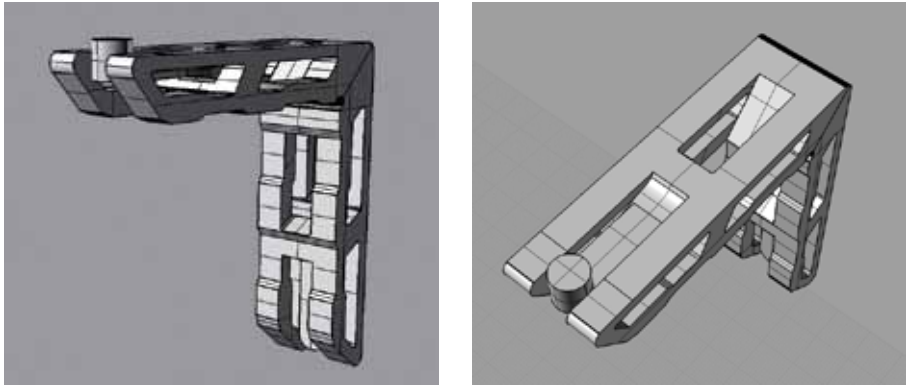
Figure 57 Rendering of part detail: 272.xx, AM optimized solution; digitally reduced material and snap-on features for additional fixation in the Aluminium profiles; digitally drawn from e-catalogue.
