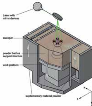
Figure 13 Schematic drawing: LS method
