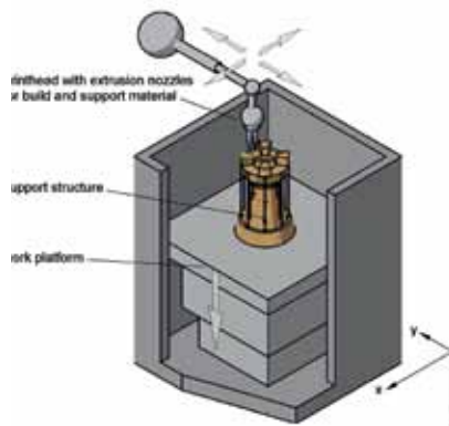
Figure 15 Schematic drawing: FDM method
